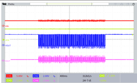
Over current protection
