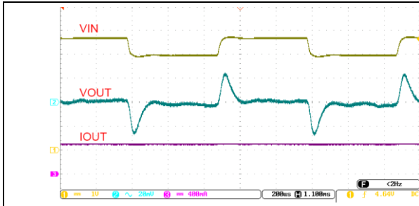
Figure 1 Line Transient ( V_{IN} =from V_{OUT}+1V to 7V to V_{OUT}+1V , I_{OUT}=0.5A )
