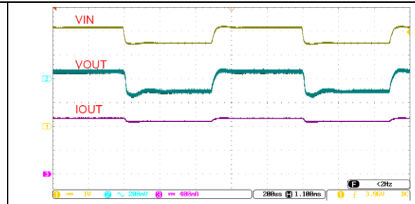
Figure 2 Line Transient ( V_{IN} =from V_{OUT}+1V to 7V to V_{OUT}+1V , I_{OUT}=1A )
