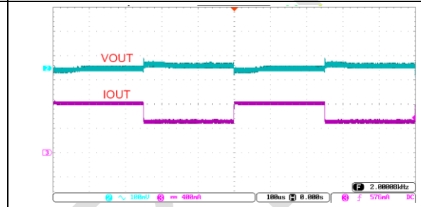
Figure 4 Load Transient ( V_{IN}=V_{OUT}+1V , I_{OUT}=0.5A-1A-0.5A )
