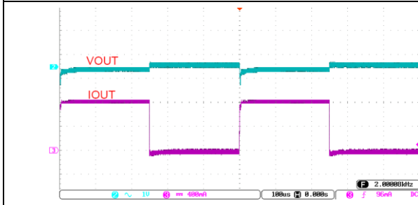
Figure 3 Load Transient ( V_{IN}=V_{OUT}+1V , I_{OUT}=0A-1A-0A )
