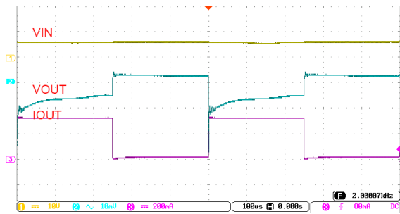
Figure 3 Load Transient (VIN=7V, IOUT=0mA-300mA-0mA)
