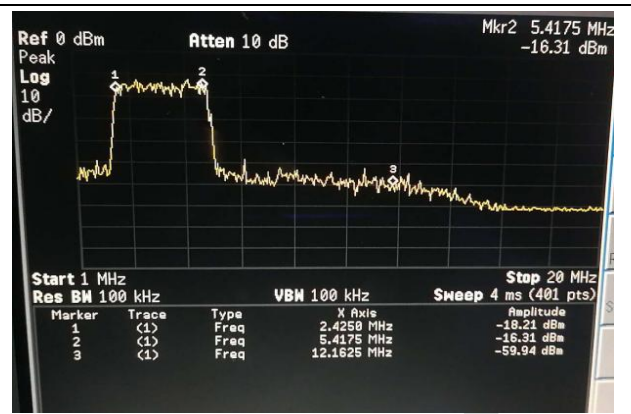
2.4MHz-5.6MHz OFDM signal transmission spectrum
