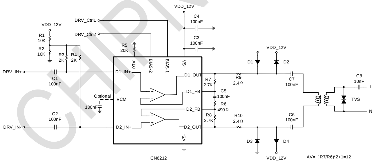
Figure 2 Typical Application
