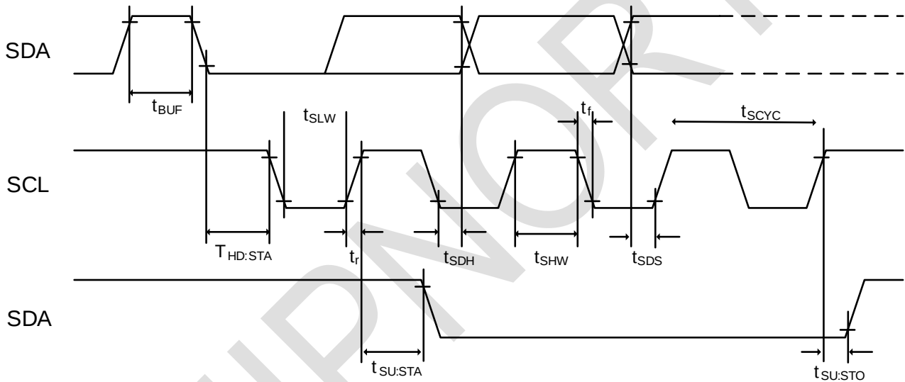
2-line serial interface timing
